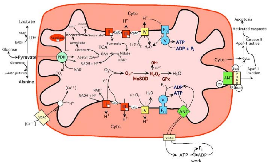
Fig. 1. Superoxide production in mitochondria, cited from (Raha & Robinson, 2000)
